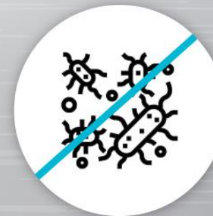
Anti-bacterial Effect
